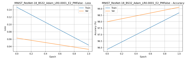
Fig. 1. Training curves for best MNIST model (ResNet-18, BS=32, Adam, LR=0.0001)
