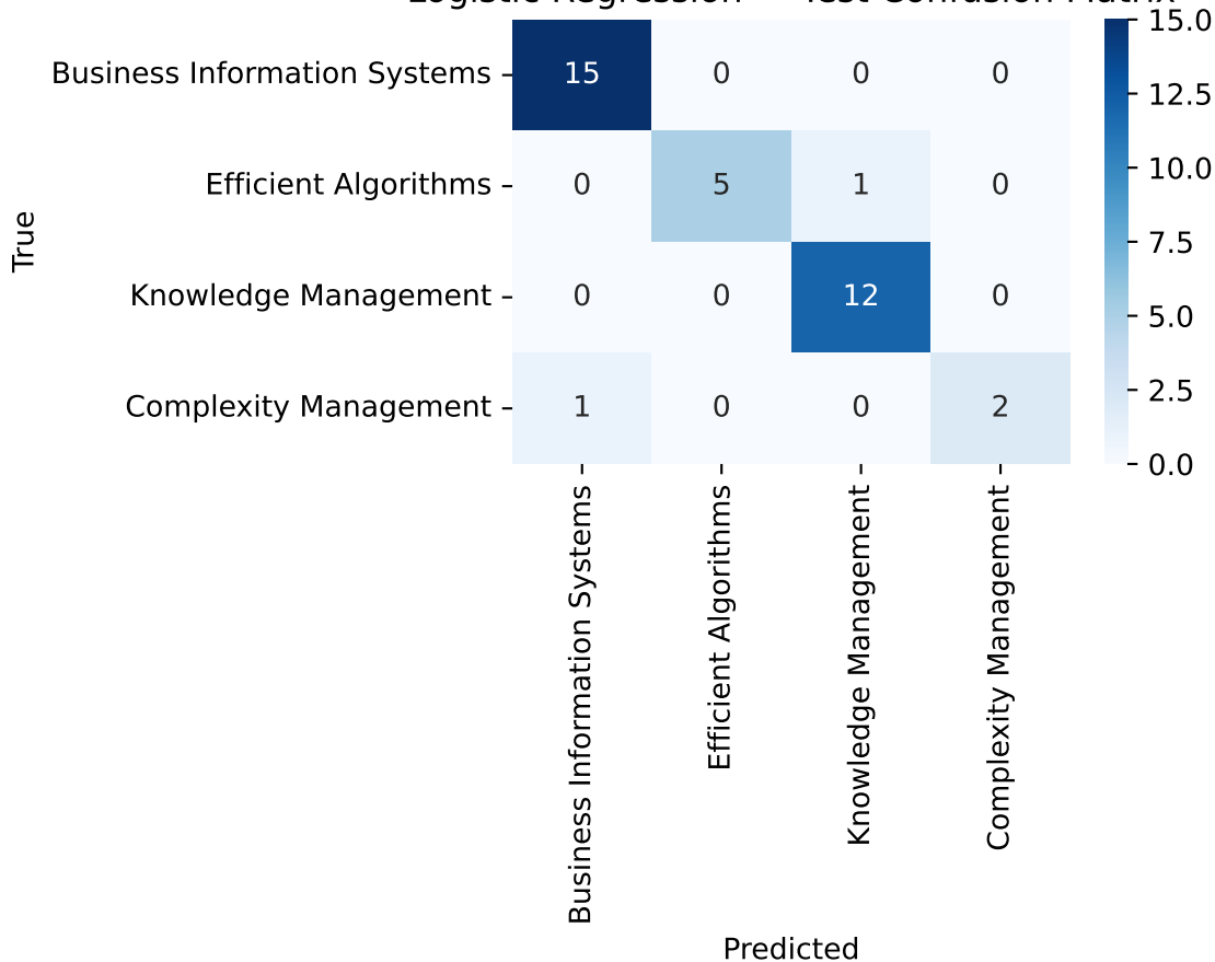
Logistic Regression — Test Confusion Matrix
