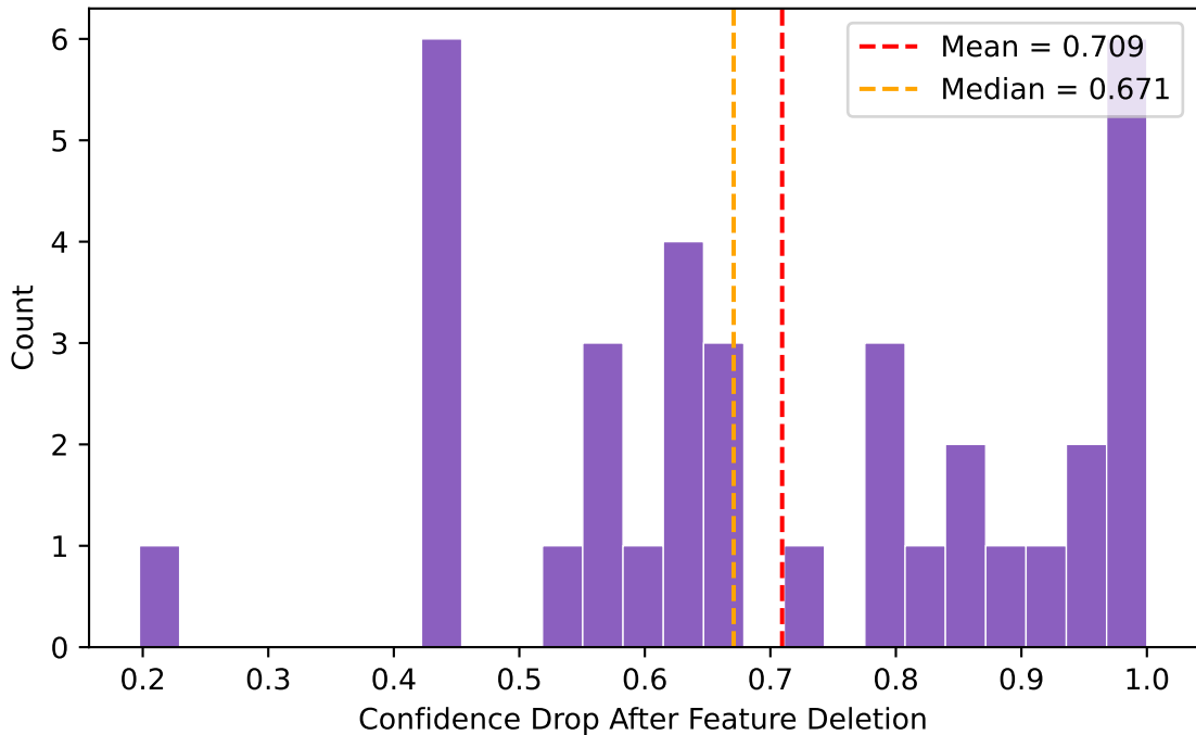
Faithfulness: Confidence Drop Distribution
