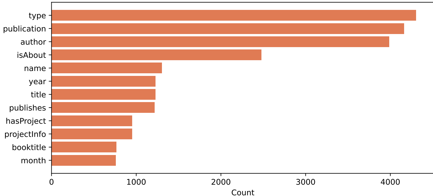
Most Frequent Predicates in AIFB
