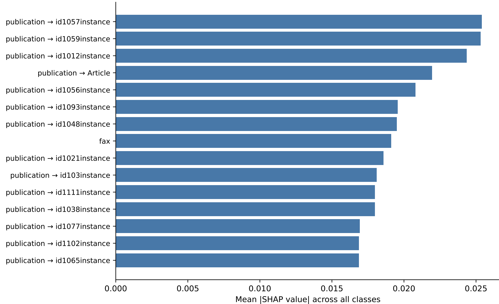
Global Feature Importance (SHAP) Top 15 features — AIFB Research Group Classification
