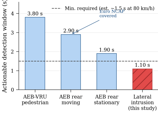
Fig. 10. Response windows: Euro NCAP longitudinal scenarios provide 1.9–3.8 s of actionable time; the lateral intrusion scenario provides 1.10 s—after sensors had already detected the threat 3 seconds earlier.
