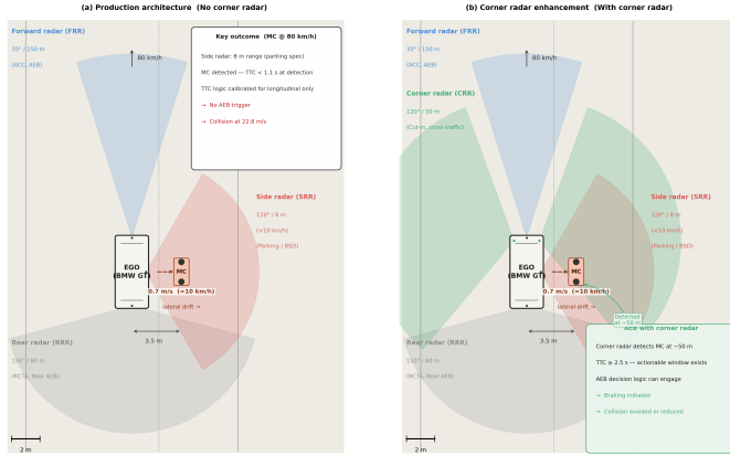
Fig. 3. Production sensor architecture (left) exhibits lateral blind zone from 35° forward FOV and parking-spec side radar; corner radar enhancement (right) restores lateral coverage.
