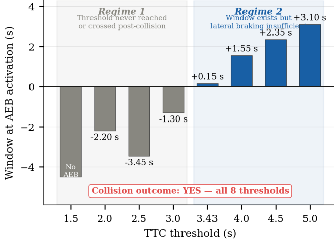
Fig. 8. TTC threshold sensitivity (1.5–5.0 s): collision outcomes in all eight configurations, confirming failure is architectural and TTC-independent.
