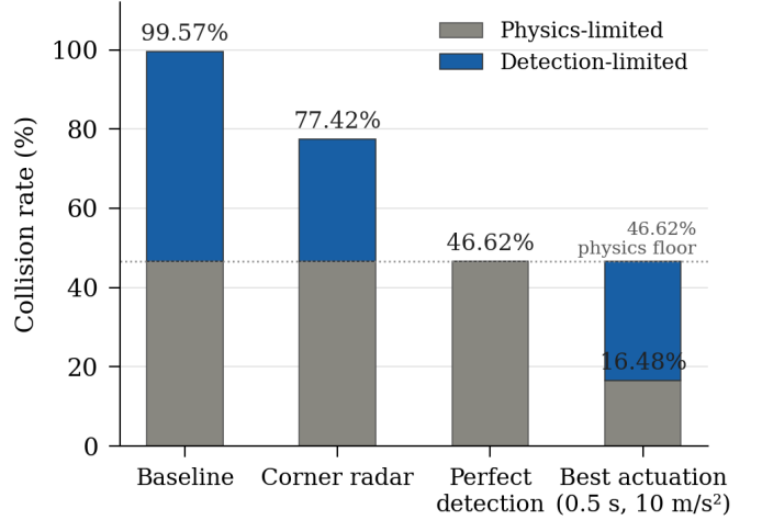
Fig. 12. Failure attribution: 53.2% of collisions are detection-limited and addressable through sensor architecture improvement. The remaining 46.6% are physics-limited and unavoidable under the modelled lateral kinematics at 80 km/h.
