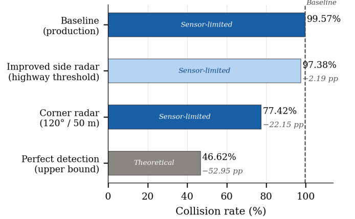
Fig. 11. Counterfactual comparison: corner radar reduces collisions by 22.15 pp— 10.1\times more than the side radar upgrade (2.19 pp). Range and field-of-view both matter.
