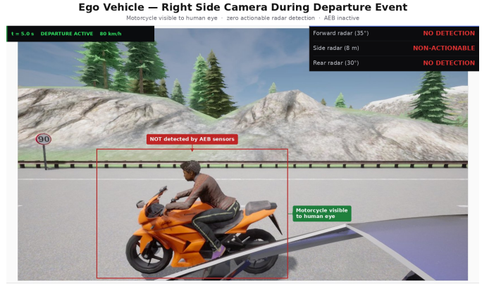
Fig. 4. CARLA frame at t = 5.0 s: motorcycle visible but zero actionable detection (forward FOV gap, side radar non-actionable at highway speed).
