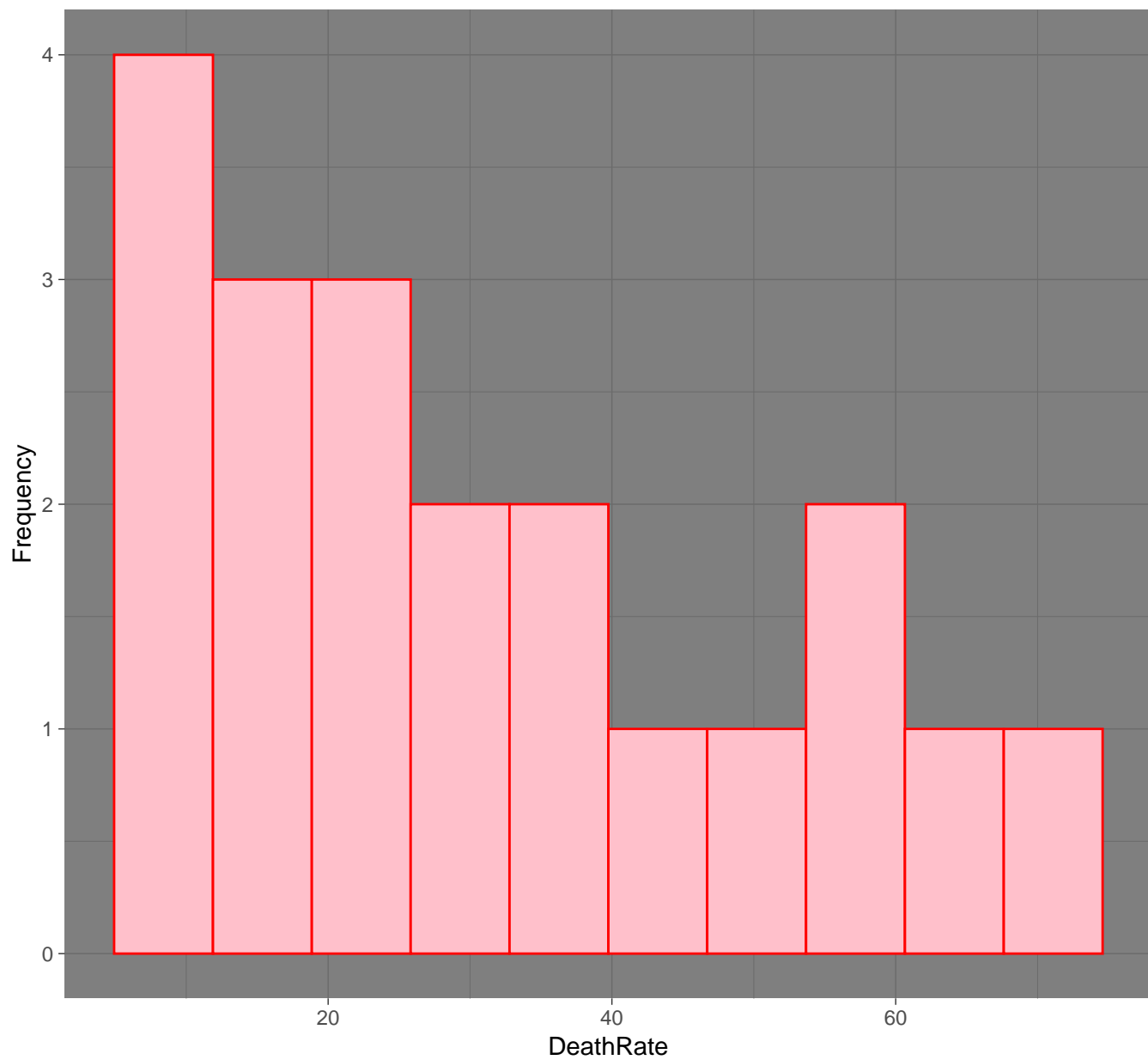
GGPLOT-Histogram
