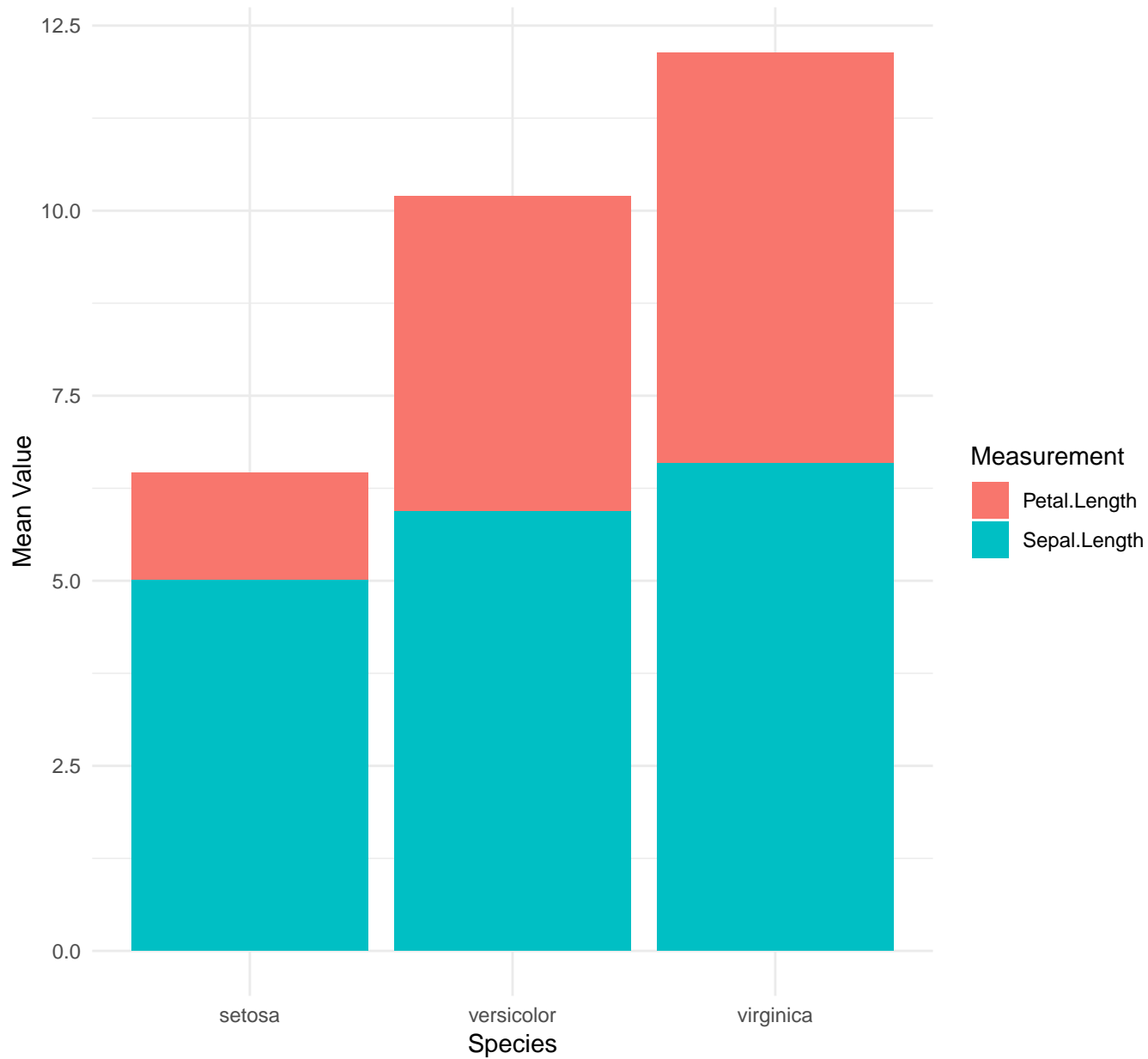
Stacked Bar Chart of Mean Measurements (Iris)
