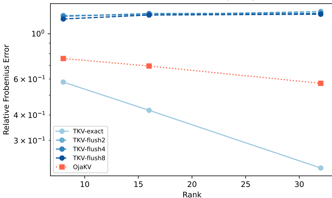
Reconstruction Error (t=256)
