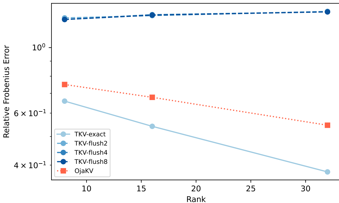
Reconstruction Error (t=512)
