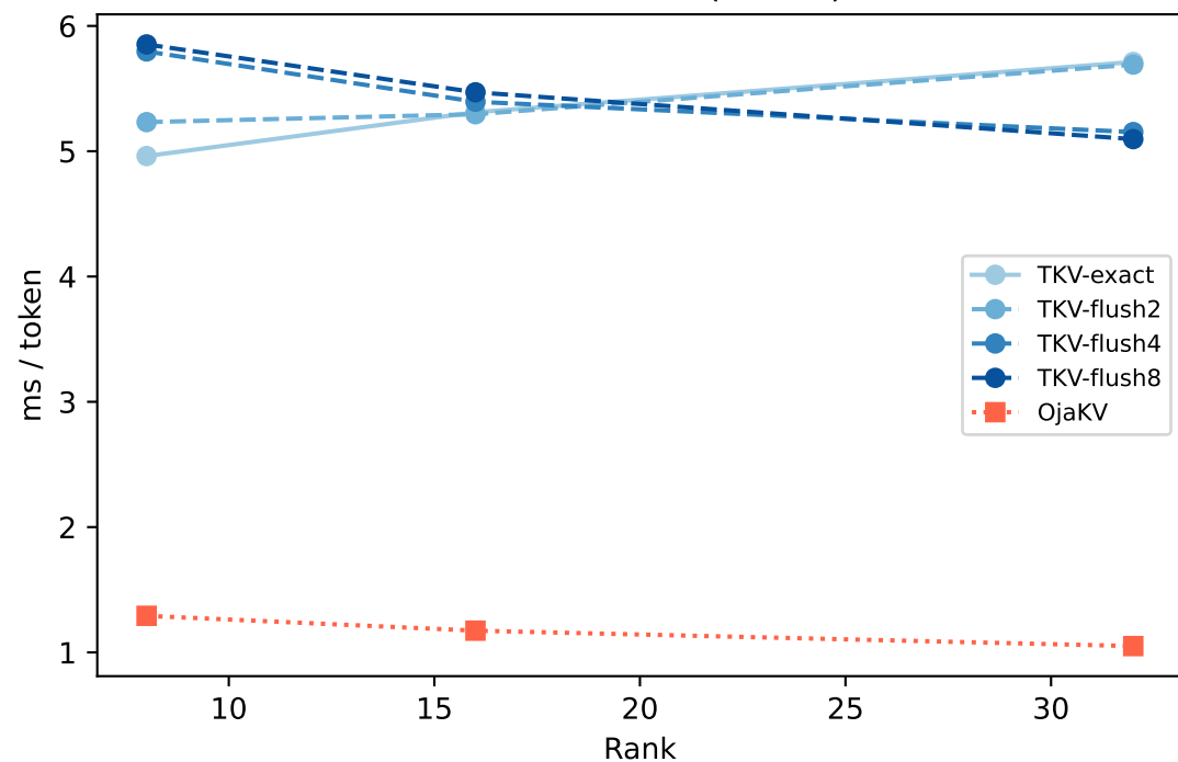
Per-Token Time (t=512)
