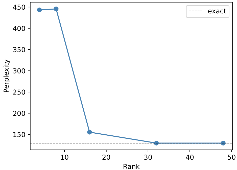
GPT-2 Perplexity vs KV Cache Rank
