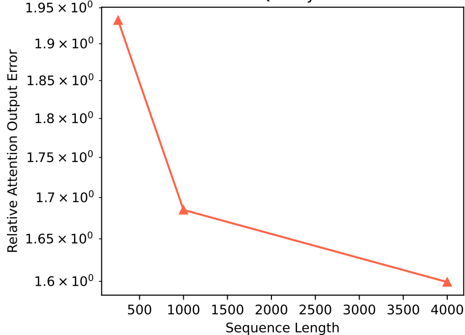
Sunked Attention Quality vs Frozen Basis
