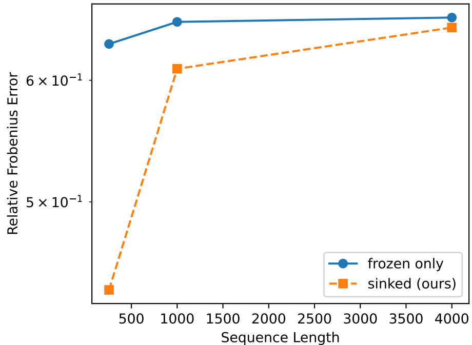
Total Reconstruction Error: Frozen vs Sinked
