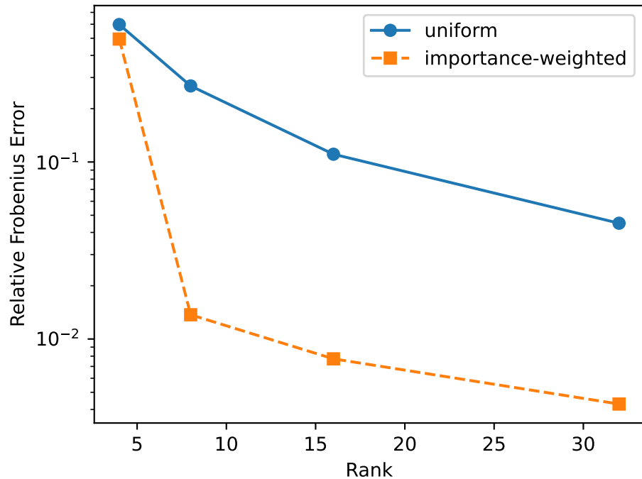
Important-Token Reconstruction Error vs Rank
