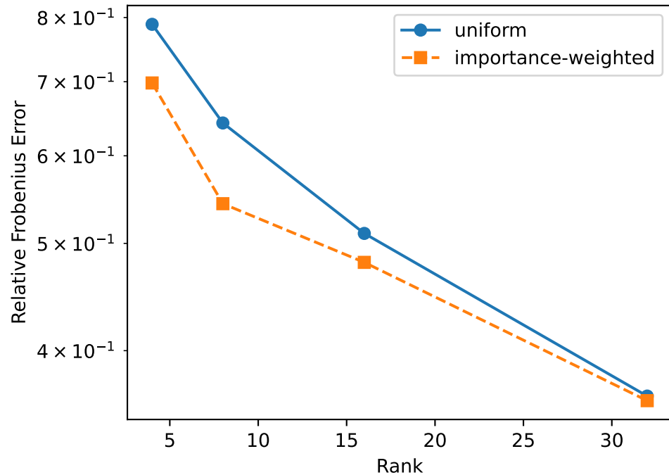
Total Reconstruction Error vs Rank
