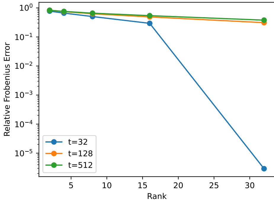
Reconstruction Error vs Rank
