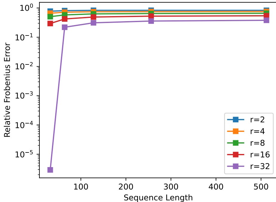
Reconstruction Error vs Sequence Length
