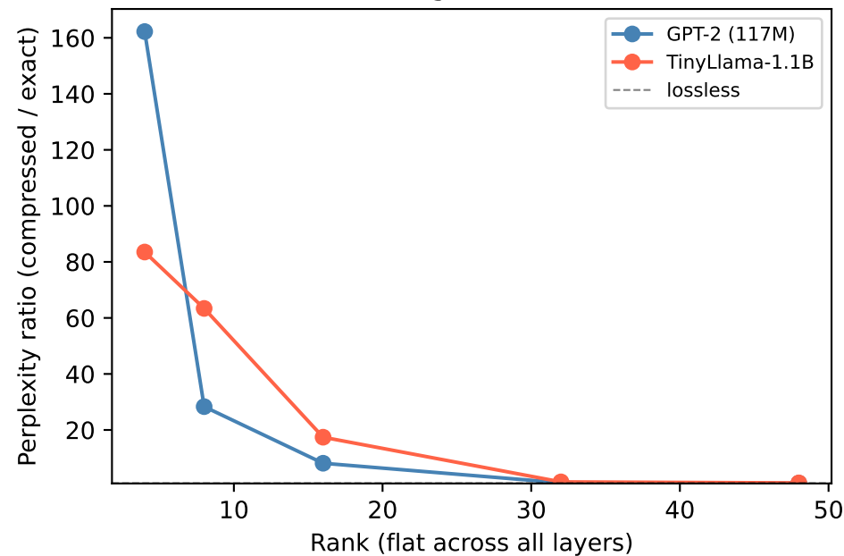
Context length = 512 tokens
