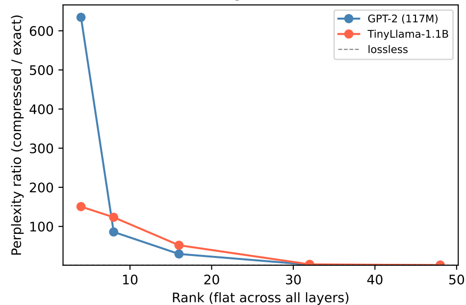
Context length = 1024 tokens
