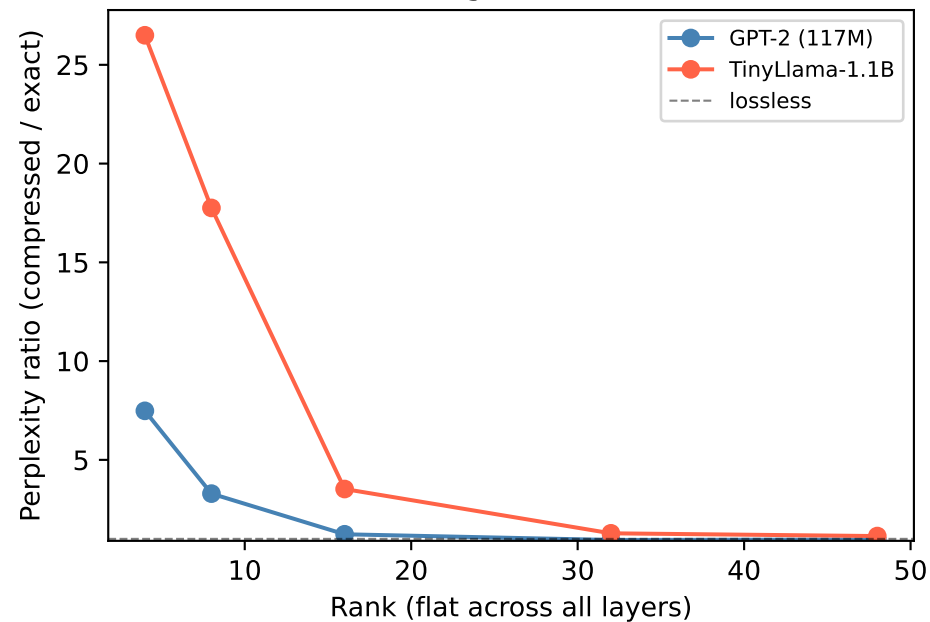
Context length = 128 tokens
