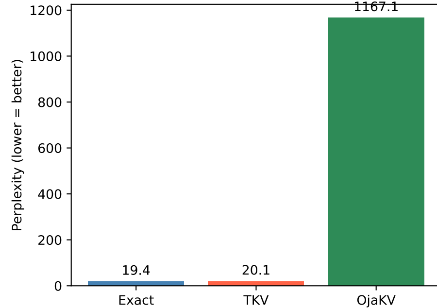
GPT-2 Perplexity Comparison
