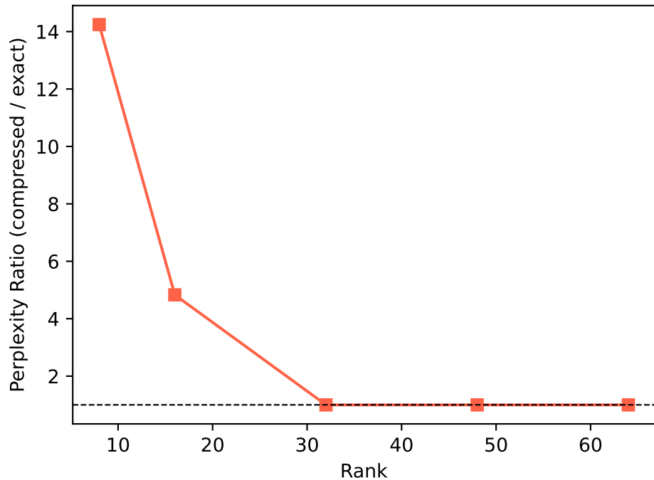
Perplexity Degradation vs Rank
