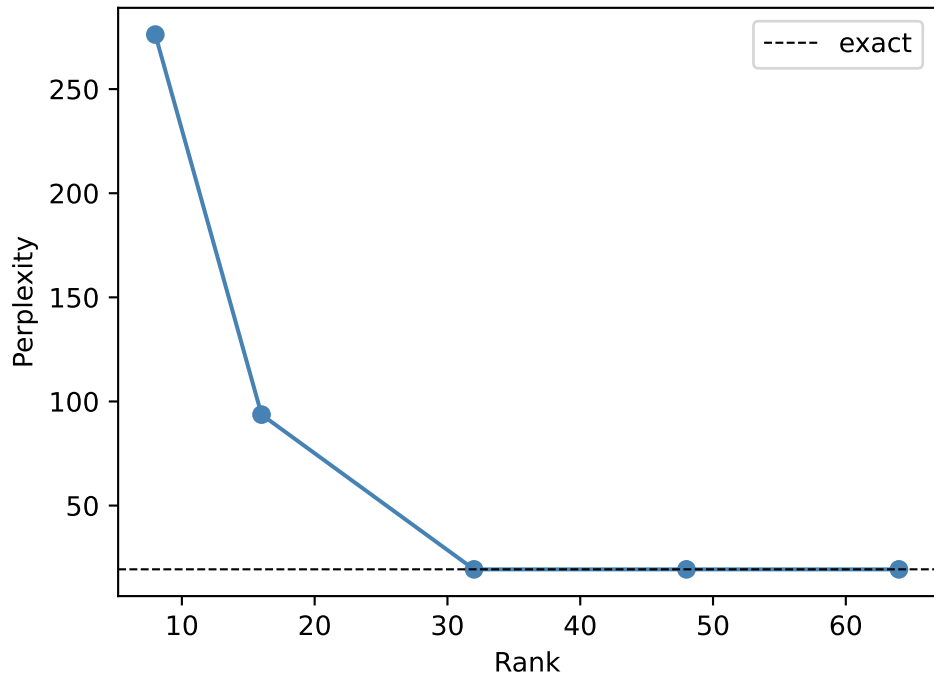
GPT-2 Perplexity vs KV Cache Rank
