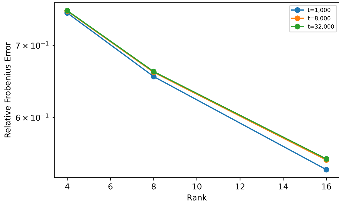
TKV Error vs Rank
