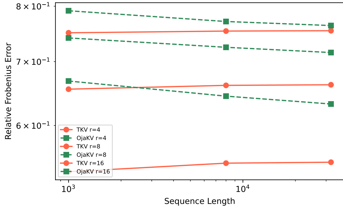
TKV vs OjaKV: Reconstruction Error
