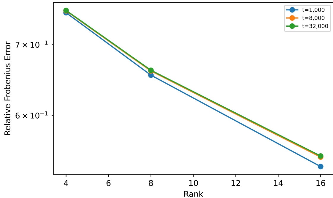
Frozen Basis Error vs Rank
