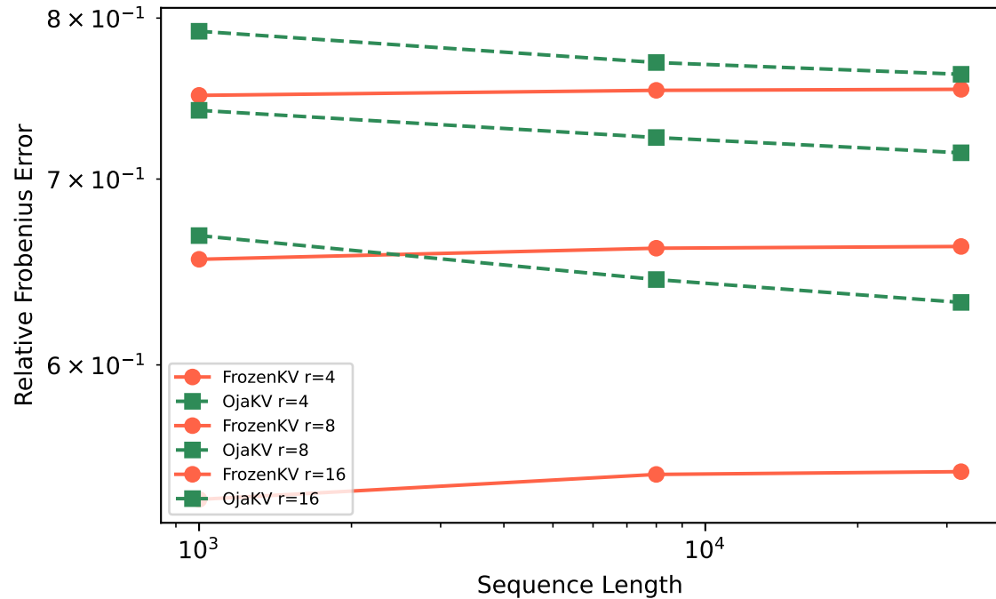
Frozen Basis vs OjaKV: Reconstruction Error
