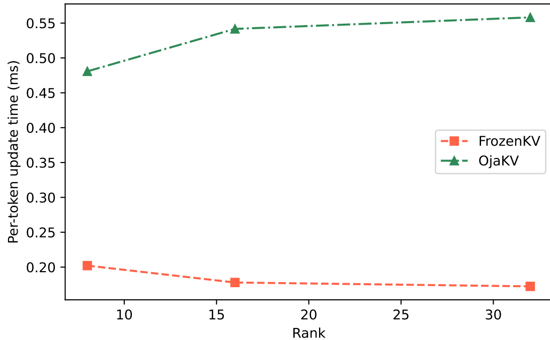
Decode-Phase Update Cost vs Rank
