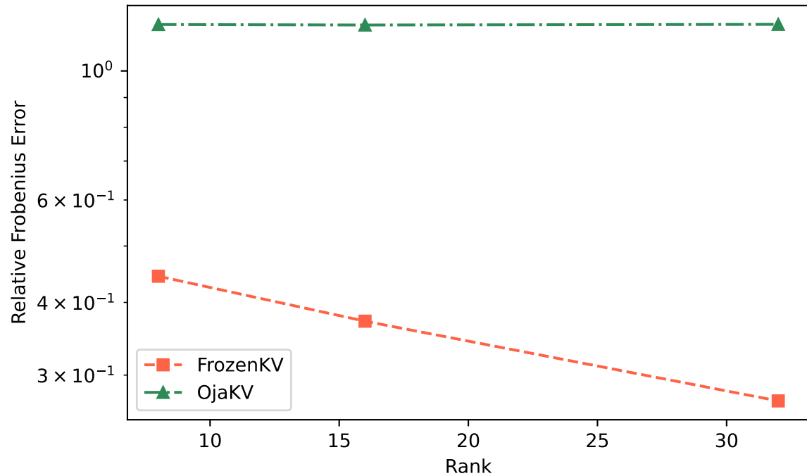
Decode-Phase Reconstruction Error vs Rank
