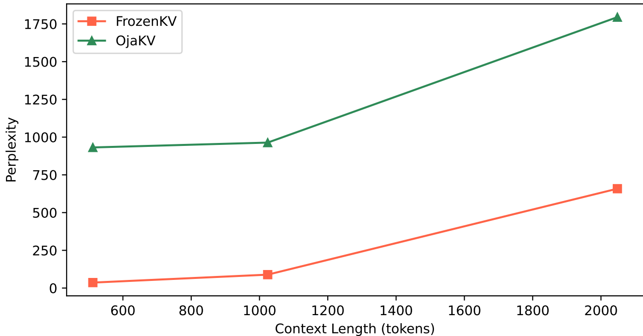
Long-Context Perplexity on WikiText-2
