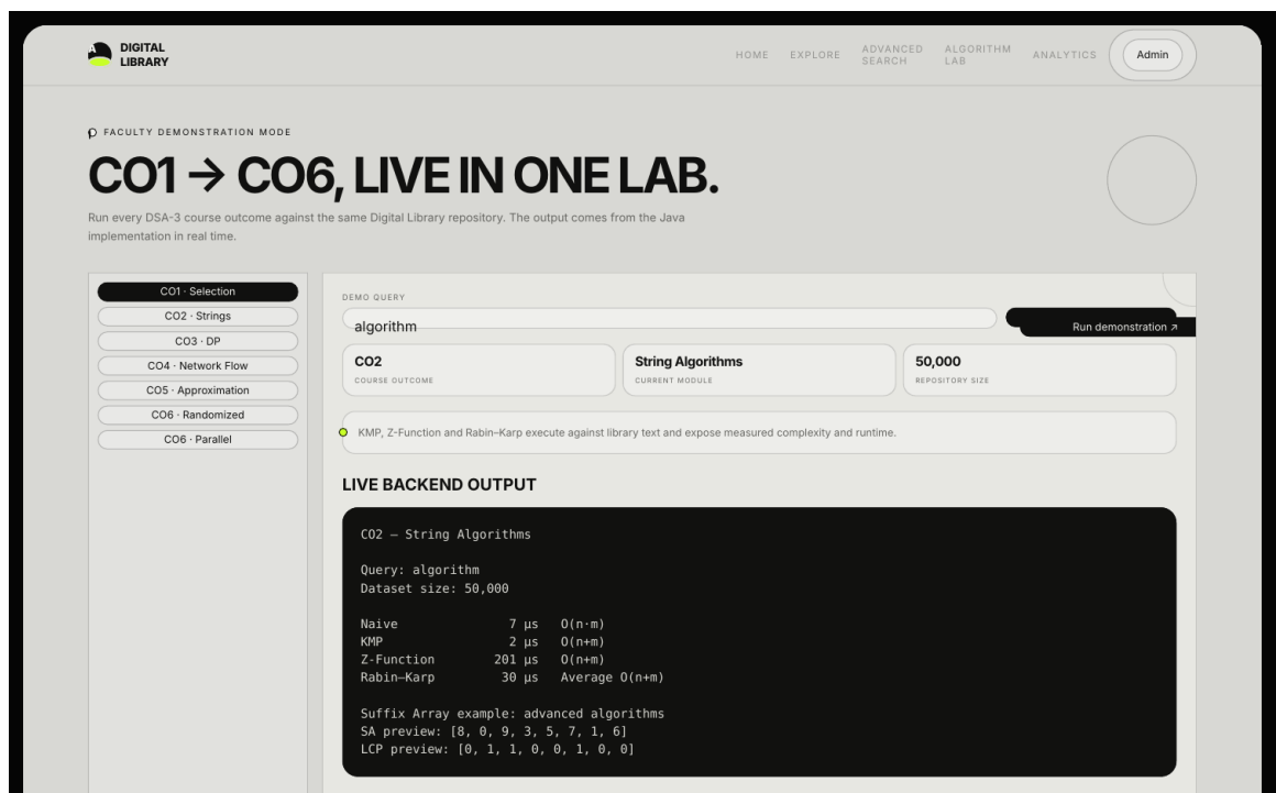
Fig. 5.3 CO1-CO6 Algorithm Lab Interface
