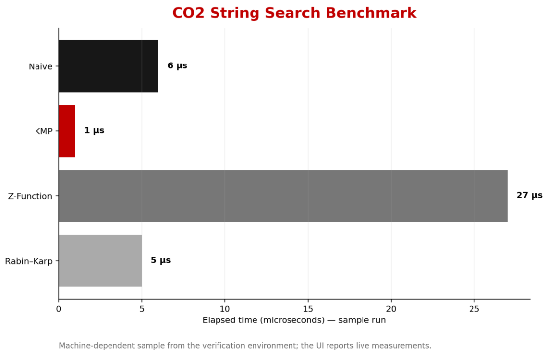
Fig. 5.5 Sample CO2 String Search Benchmark
