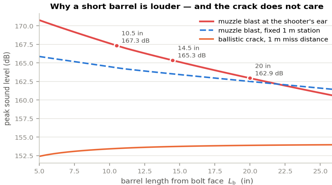
Figure 11 — Peak sound level against barrel length. The blast falls steadily as the barrel lengthens; the crack is almost perfectly flat because it depends on Mach number only through an eighth root. The "at the ear" curve is steeper than the fixed-station curve because a shorter barrel also puts the muzzle closer to the shooter's head.
