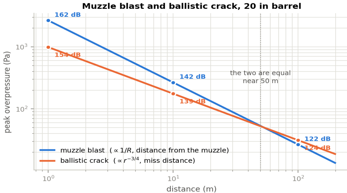
Figure 10 — The two sound sources, 20 in barrel. Note that the horizontal axis means different things for the two curves: distance from the muzzle for the blast, perpendicular miss distance from the trajectory for the crack. The shallower slope of the crack is the whole story.
