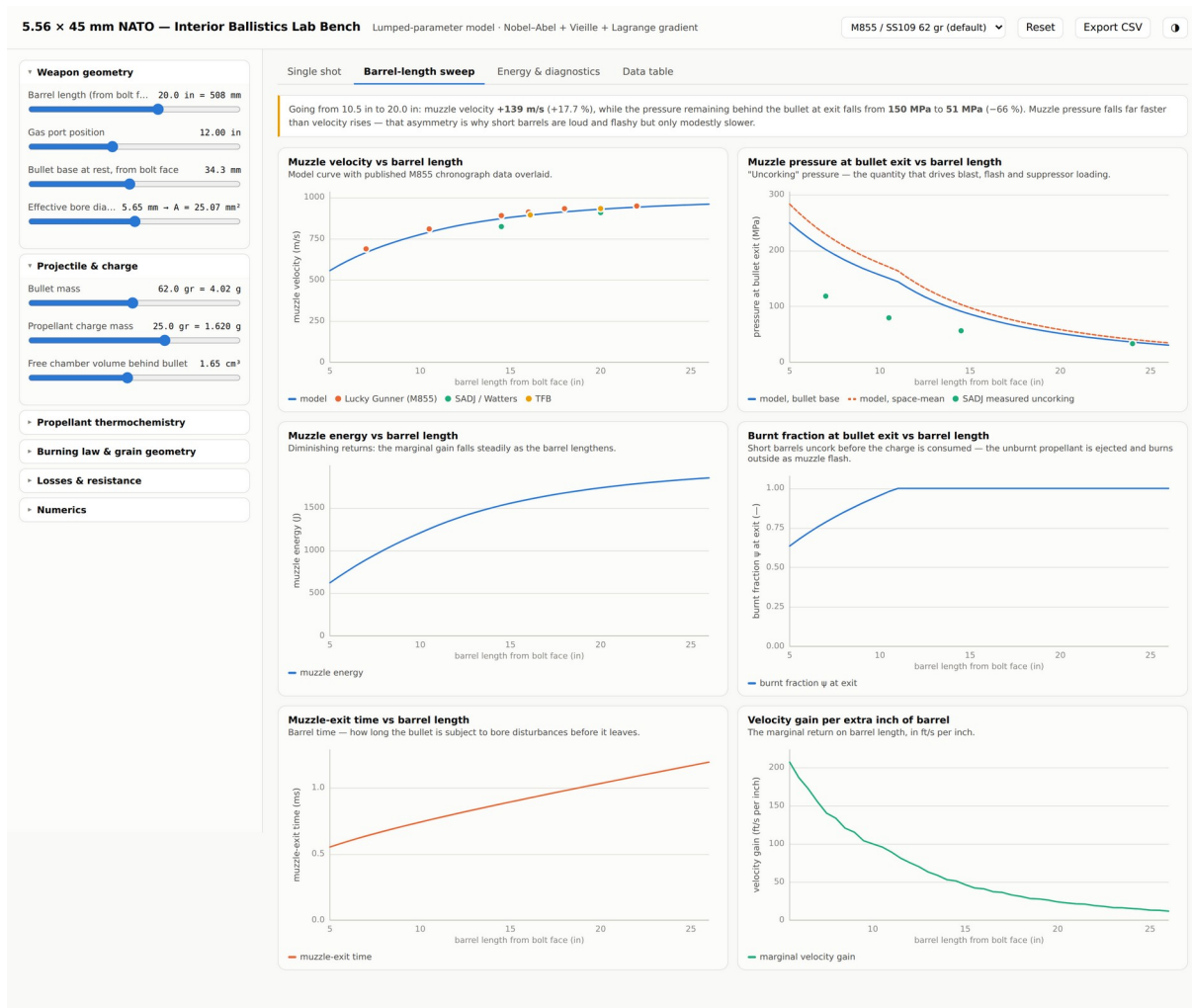
Figure 10 — The barrel-length sweep tab, with published chronograph and uncorking-pressure measurements overlaid on the model curves.
