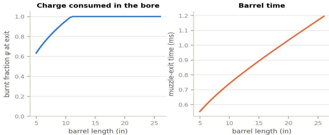
Figure 8 — Left: the fraction of the charge consumed before the bullet exits. Below about 11.5 in the round leaves the barrel with propellant still burning. Right: barrel time, which grows almost linearly with barrel length.
