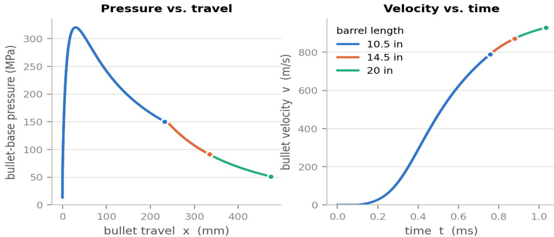
Figure 7 — Left: bullet-base pressure against bullet travel — the area under each curve, multiplied by the bore area, is the work delivered to the bullet. Right: velocity against time, showing how the acceleration has already fallen to a small value long before the muzzle of a long barrel.
