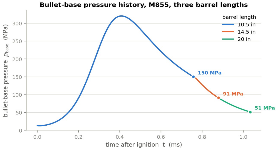
Figure 6 — Bullet-base pressure history for three barrel lengths. The three curves are identical until the shortest barrel uncorks: barrel length does not change the pressure history, it only decides where on that history the bullet leaves. The end point of each curve is its muzzle pressure.
