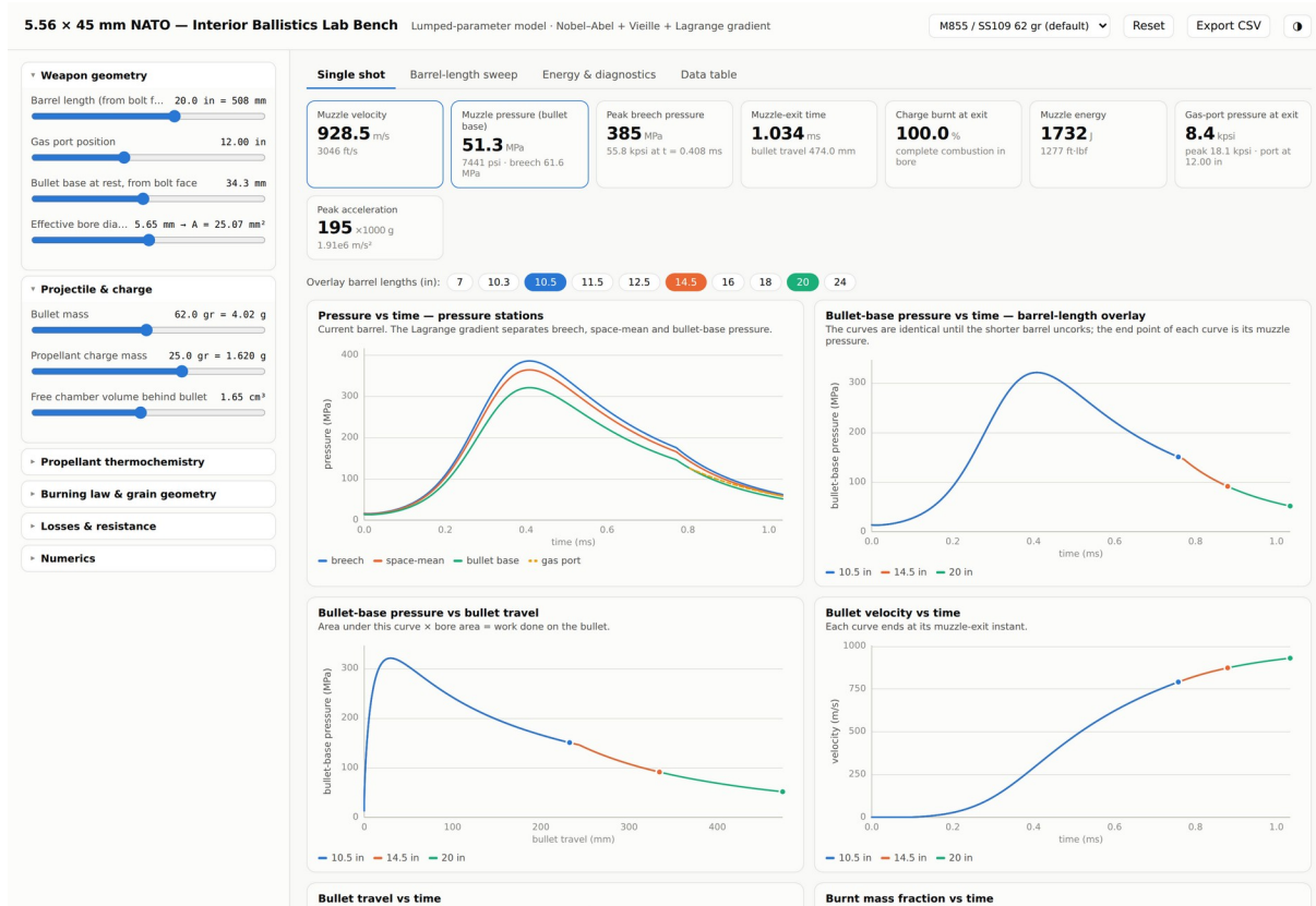
Figure 9 — The single-shot tab of the simulator. The overlaid pressure curves for 10.5 in, 14.5 in and 20 in barrels coincide exactly, each terminating at its own muzzle-exit point.
