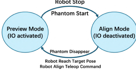
Fig. 6: State Transition of Preview Control
