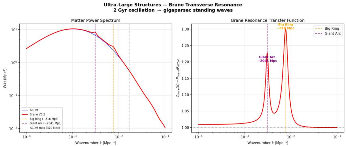
Figure: Brane transverse resonance produces clustering peaks at k_1 = 816 Mpc and k_2 = 2041 Mpc, both exceeding CDMs maximum structure size (370 Mpc). The fundamental resonance scale matches the Big Ring observation at z = 0.8 .
