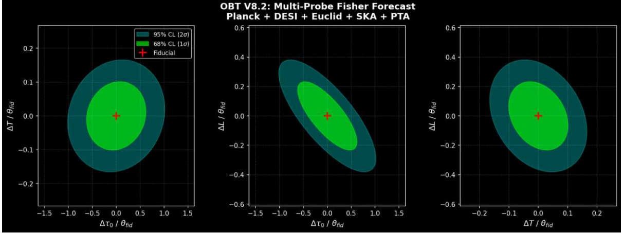
Figure: Multi-probe Fisher forecast for OBT V8.2. Confidence ellipses at 68% CL (green) and 95% CL (cyan) in the three 2D parameter planes. The \theta - L anti-correlation is broken by the PTA cross-constraint.
