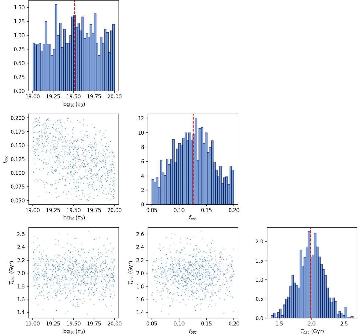
Figure: Nested sampling posteriors ( dynesty ) for the brane parameters. Original 3-parameter run: \ln K \in [2.8, 4.13] . After Chronological Anchoring ( T derived, 2-parameter model): \ln K approximately 5.8 ( Decisive ).
