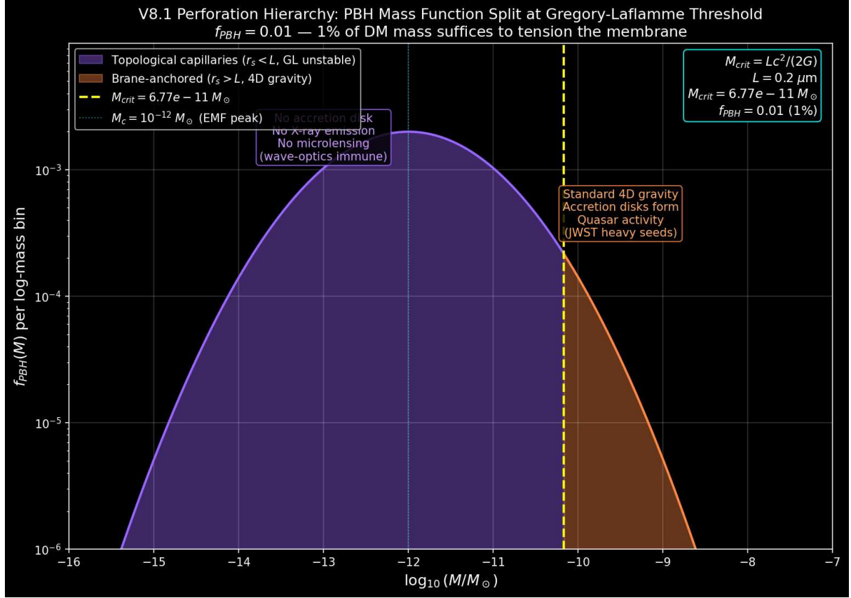
Figure: Gregory-Laflamme perforation hierarchy. PBHs below M_{crit} (purple) undergo GL instability and become 5D objects — topological capillaries invisible to accretion and microlensing. PBHs above M_{crit} (orange) remain brane-anchored with standard 4D gravity.
