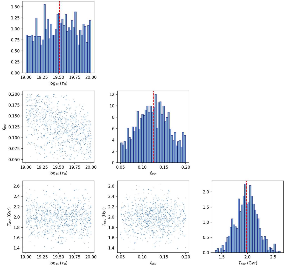
Nested Sampling Posteriors — Brane V8.2 \Delta \ln K = 4.09 \pm 0.07 ( STRONG )
