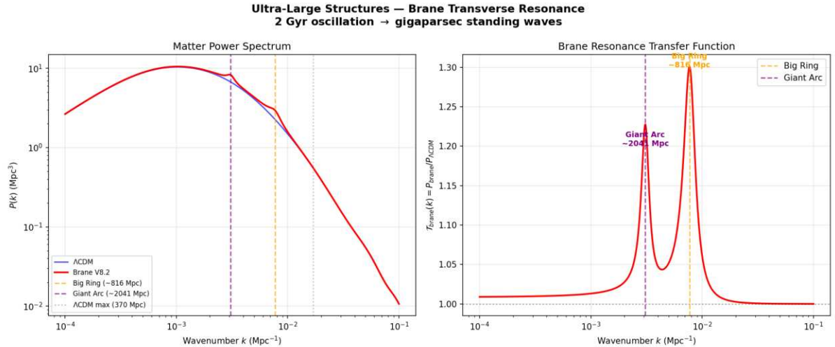
Figure: Brane transverse resonance produces clustering peaks at \lambda_1 = 816 Mpc and \lambda_2 = 2041 Mpc, both exceeding CDMs maximum structure size (370 Mpc). The fundamental resonance scale matches the Big Ring observation at z = 0.8 .
