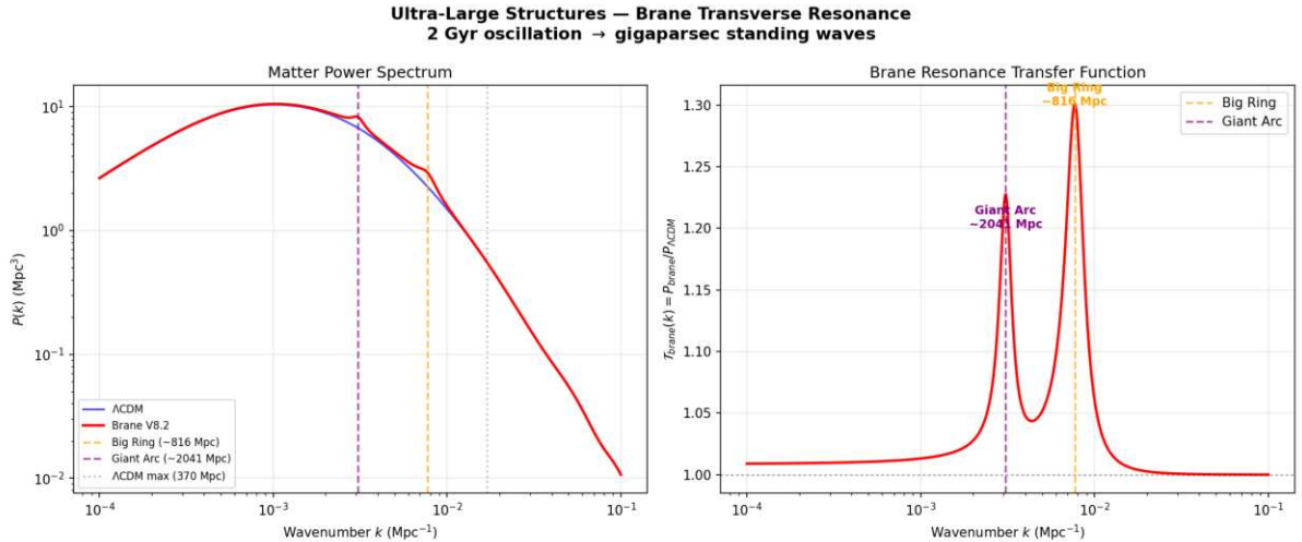
Figure: Brane transverse resonance produces clustering peaks at \lambda_1 = 816 Mpc and \lambda_2 = 2041 Mpc, both exceeding CDMs maximum structure size (370 Mpc). The fundamental resonance scale matches the Big Ring observation at z = 0.8 .
