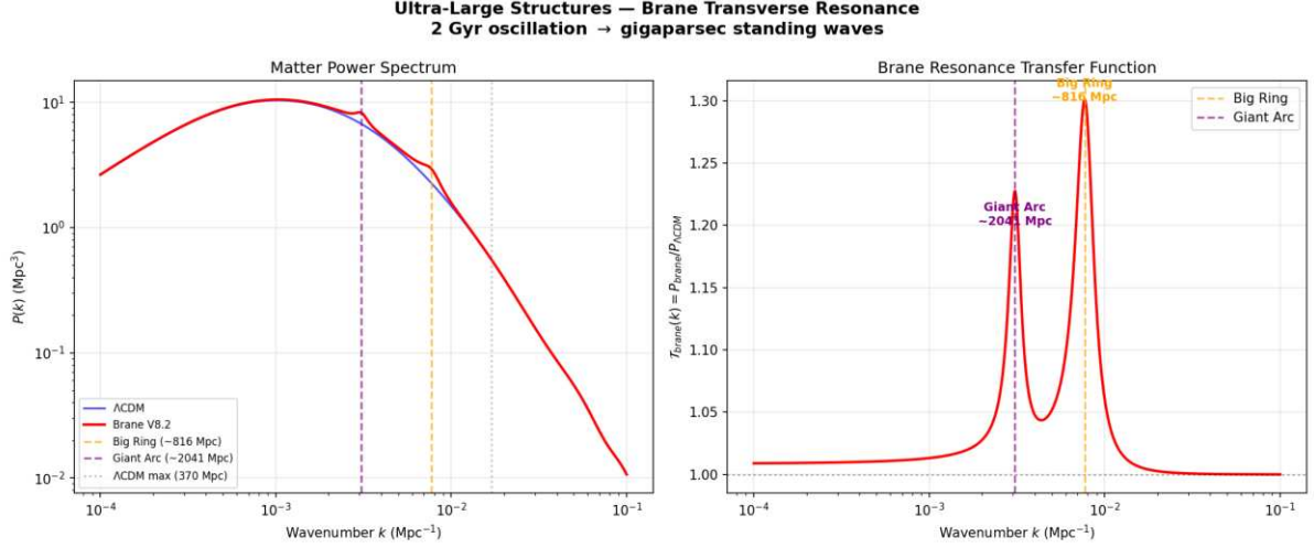
Figure: Brane transverse resonance produces clustering peaks at \sim 816 Mpc and \sim 2041 Mpc, both exceeding CDMs maximum structure size (370 Mpc). The fundamental resonance scale matches the Big Ring observation at z \sim 0.8 .
