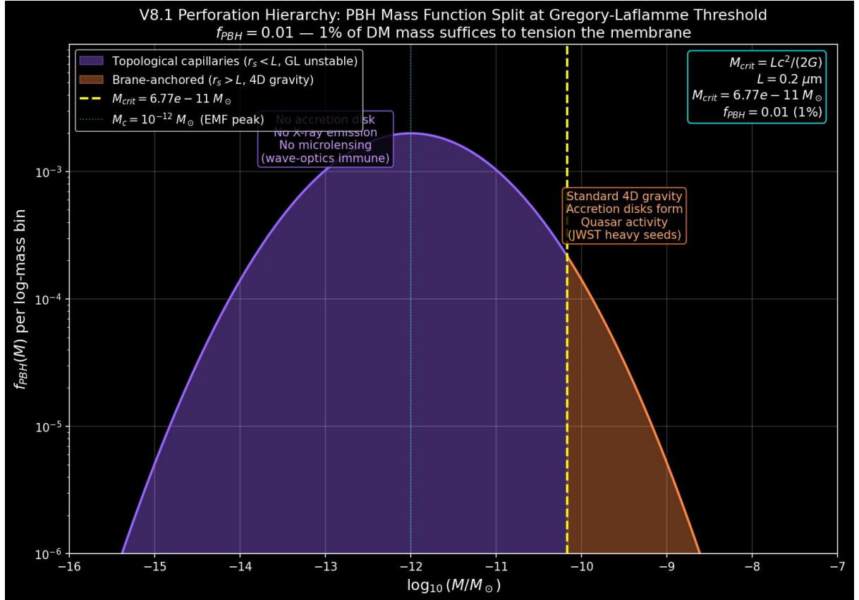
Figure: Gregory-Laflamme perforation hierarchy. PBHs below M_{crit} (purple) are 5D localized objects — topological capillaries invisible to optical microlensing (and X-ray dark by standard low-Bondi accretion). PBHs above M_{crit} (orange) remain brane-anchored with standard 4D gravity.
