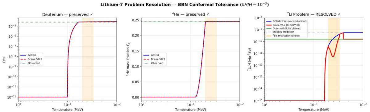
Figure: BBN conformal tolerance addresses the Lithium-7 problem. {}^7\text{Li} suppressed by 3.5\times
