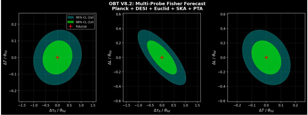
Figure: Multi-probe Fisher forecast for OBT V8.2. Confidence ellipses at 68% CL (green) and 95% CL (cyan) in the three 2D parameter planes. The \tau_0 - L anti-correlation is broken by the PTA cross-constraint.
