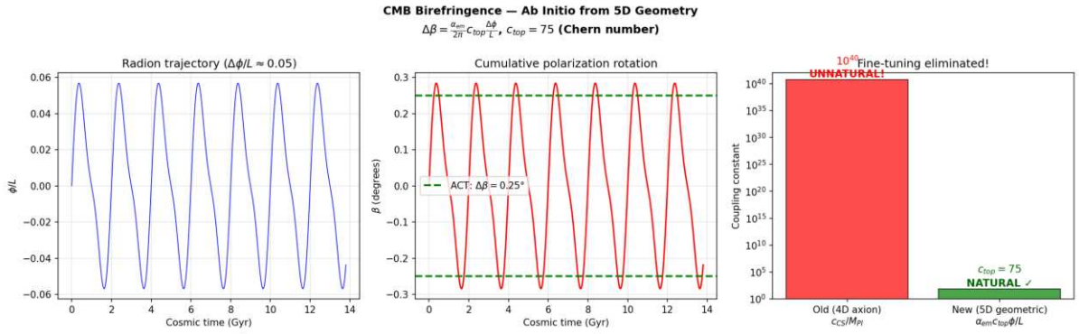
Figure: Ab initio CMB birefringence from 5D geometry. The 4D axion approach required an unnatural c_{CS} \approx 10^{40} ; the correct 5D geometric formula gives c_{top} = 75 (natural O(10^2) Chern number). \Delta\beta \approx 0.25^\circ matches ACT/Planck.
