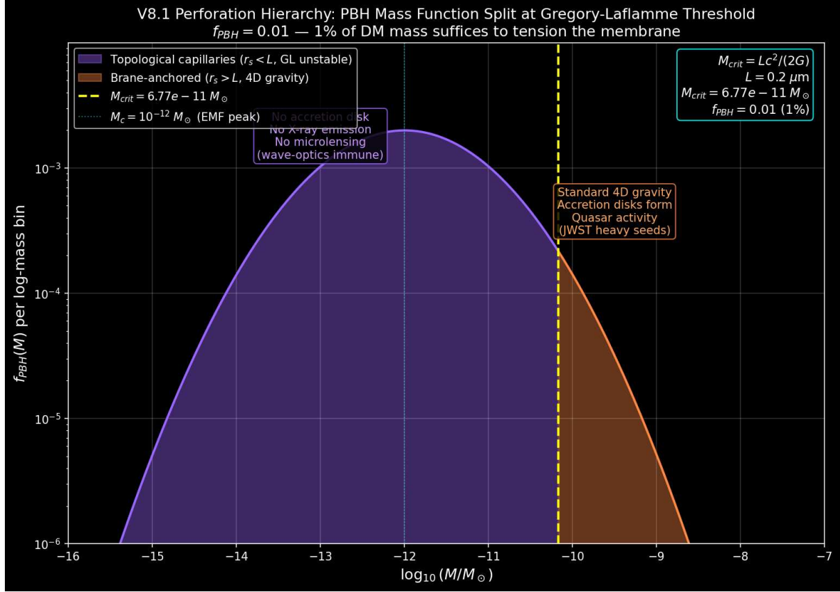
Figure: Gregory-Laflamme perforation hierarchy. PBHs below M_{\text{crit}} (purple) undergo GL instability and become 5D objects: topological capillaries invisible to accretion and microlensing. PBHs above M_{\text{crit}} (orange) remain brane-anchored with standard 4D gravity.
