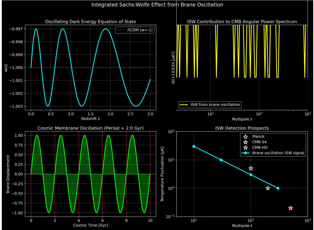
Figure 3: Theoretical prediction of ISW effect from membrane oscillations.
