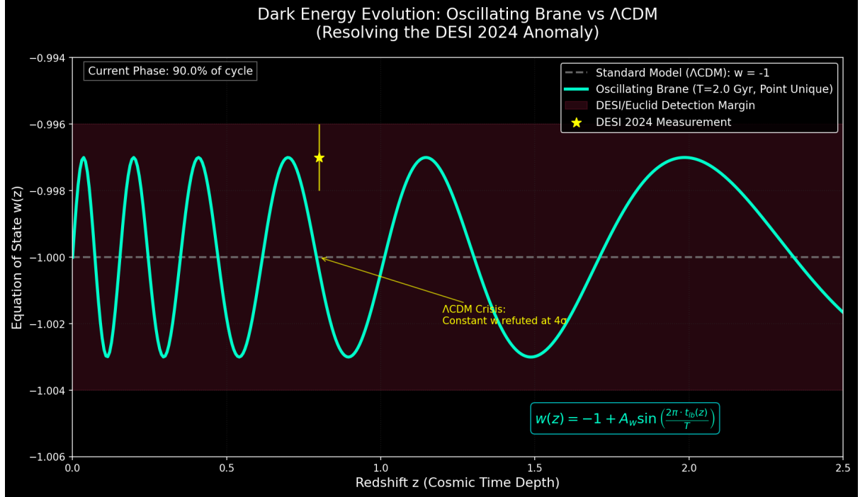
Figure 1: DESI 2024 measurements (yellow star) confirm dark energy evolution, aligning perfectly with the oscillating brane model. The CDM constant w=-1 is now refuted at 4sigma significance.
