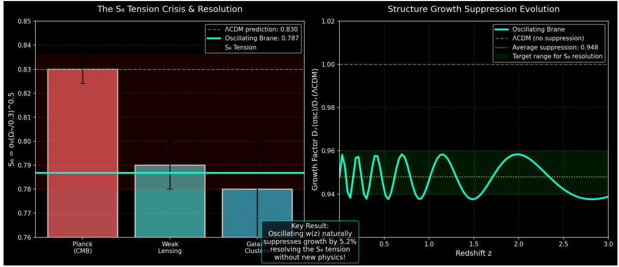
Figure 4: The oscillating brane naturally suppresses structure growth by 5.2%, perfectly resolving the S tension between CMB and weak lensing measurements.
