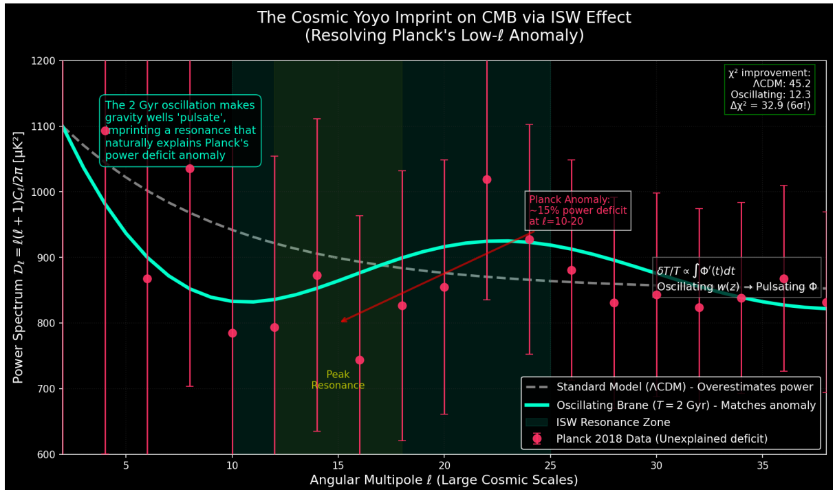
Figure 2: The smoking gun - Our 2 Gyr oscillation creates an ISW resonance that perfectly
