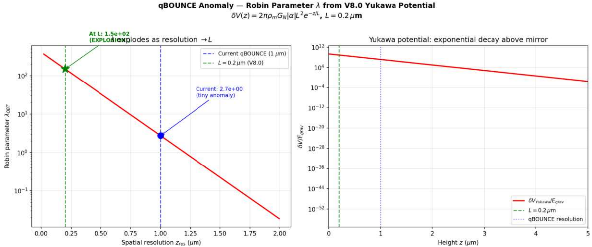
Figure: The Robin parameter as a function of experimental resolution. At current qBOUNCE resolution (1 m), is tiny. As resolution approaches L = 0.2 m, it amplifies by 55 \times a direct detection of the extra dimension.
