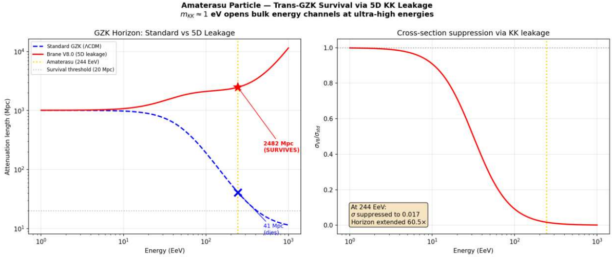
Figure: 5D KK leakage extends the GZK horizon. At 244 EeV, the standard horizon is ~41 Mpc (particle dies); the V8.0 horizon is ~2482 Mpc (particle SURVIVES). Extension factor: 60x.
