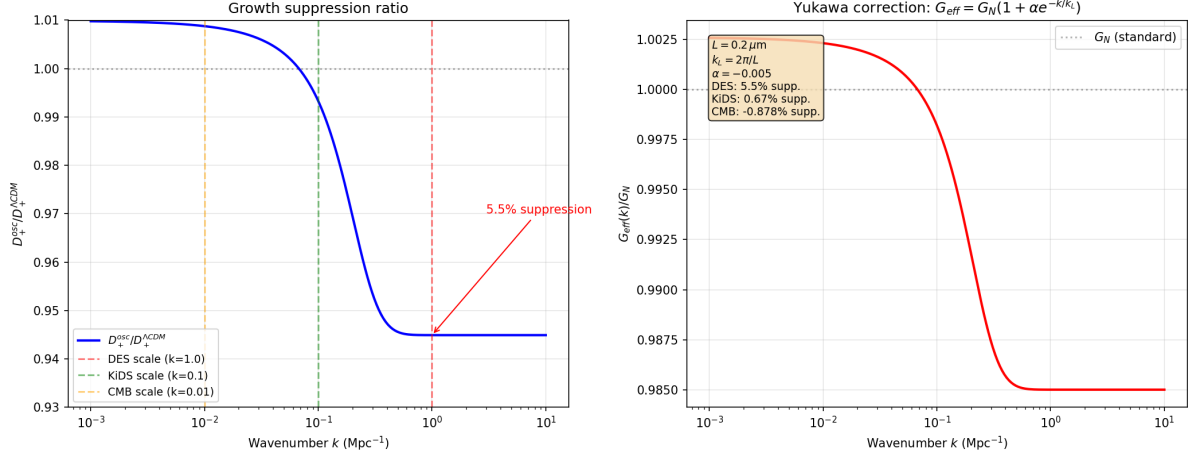
Figure: Scale-dependent growth suppression via Yukawa screening. DES non-linear scales show \sim 5.5\% suppression ( S = 0.790 ), while KiDS/CMB linear scales remain quasi-standard ( < 1\% ). Computed with BDF stiff solver.
