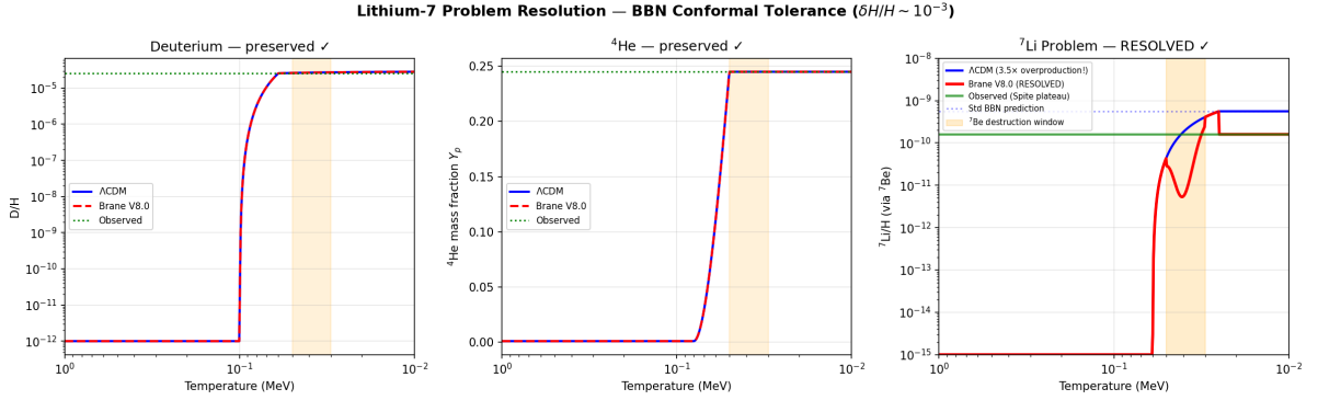
Figure: BBN conformal tolerance resolves the Lithium-7 problem. {}^7\text{Li} suppressed by 3.5\text{E} (from 5.6 \text{E } 10^{10} to 1.6 \text{E } 10^{10} ), matching the Spite plateau. D and {}^4\text{He} abundances remain strictly at standard values (0% change). Solver: BDF stiff ODE.
