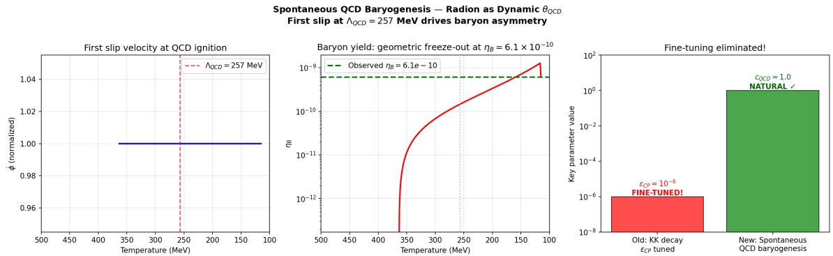
Figure: Spontaneous QCD baryogenesis via radion-driven dynamic QCD . The first slip at QCD = 257 MeV drives the baryon chemical potential, freezing out at B = 6.10 \text{E } 10^{10} . Coupling c_{QCD} = 1.0 (natural O(1) , no fine-tuning). No CP needed.
