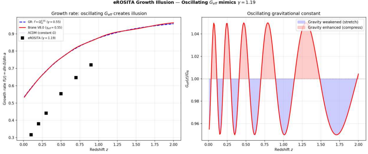
Figure: Oscillating G_{\text{eff}}(z) creates the illusion of \gamma = 1.19 when fitted with a constant- G model. The growth rate f(z) deviates from GRs_{m}^{0.55} at low redshifts where the brane is currently stretched.
