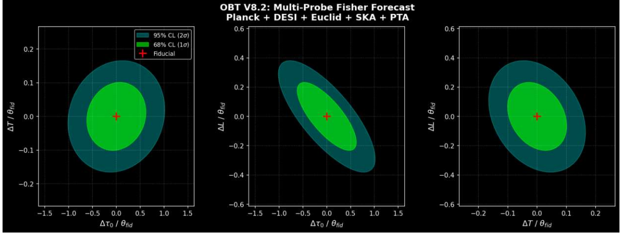
Figure: Multi-probe Fisher forecast for OBT V8.2. Confidence ellipses at 68% CL (green) and 95% CL (cyan) in the three 2D parameter planes. The {}_0 - L anti-correlation is broken by the PTA cross-constraint.
