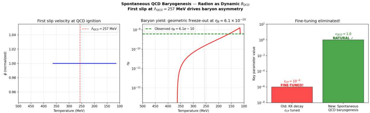
Figure: Spontaneous QCD baryogenesis via radion-driven dynamic QCD . The first slip at
