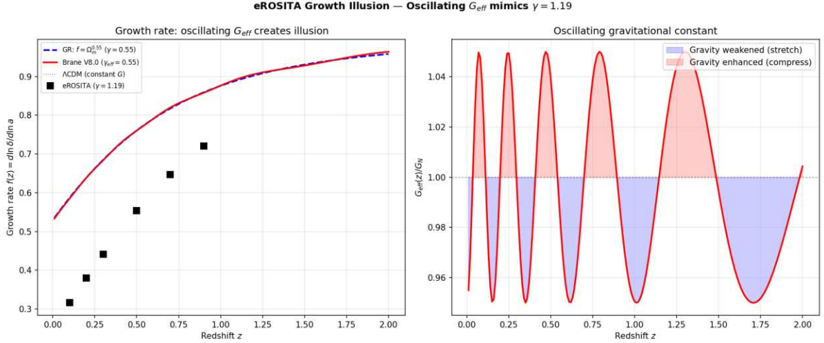
Figure: Oscillating G_{\text{eff}}(z) creates the illusion of \gamma = 1.19 when fitted with a constant- G model. The growth rate f(z) deviates from GRs \Omega_m^{0.55} at low redshifts where the brane is currently stretched.
