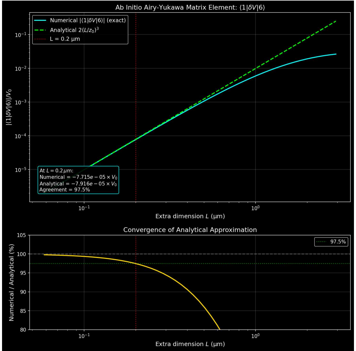
Figure: Ab initio Airy-Yukawa matrix element \langle 1|V|6 \rangle vs extra dimension size L . Cyan: exact numerical integration; green dashed: analytical limit 2V_0(L/z_0)^3 . Red line: L = 0.2 \mu\text{m} . Agreement exceeds 97% across the physical range.
