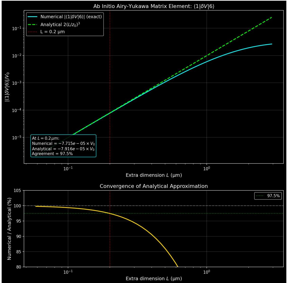
Figure: Ab initio Airy-Yukawa matrix element \langle 1|\delta V|6\rangle vs extra dimension size L . Cyan:
