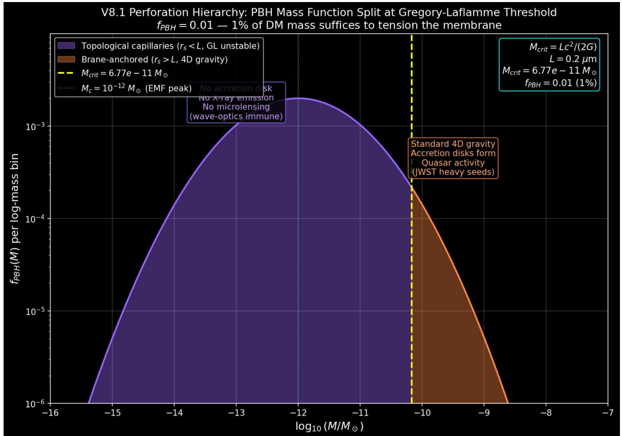
Figure: Gregory-Laflamme perforation hierarchy. PBHs below M_{crit} (purple) undergo GL
