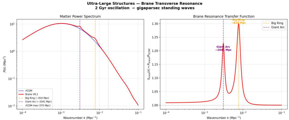
Figure: Brane transverse resonance produces clustering peaks at k_1 \approx 1/816 Mpc ^{-1} and k_2 \approx 1/2041 Mpc ^{-1} , both exceeding CDMs maximum structure size (370 Mpc). The fundamental resonance scale matches the Big Ring observation at z \approx 0.8 .
