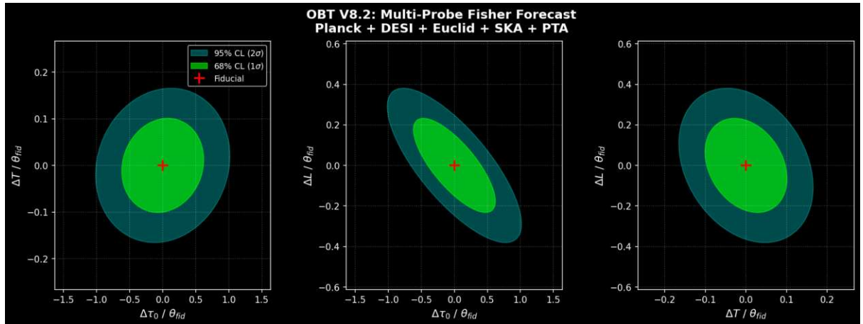
Figure: Multi-probe Fisher forecast for OB T V8.2. Confidence ellipses at 68% CL (green) and 95% CL (cyan) in the three 2D parameter planes. The 0 - L anti-correlation is broken by the
