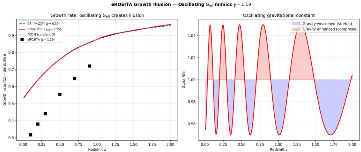
Figure: Oscillating G_{\text{eff}}(z) creates the illusion of \gamma = 1.19 when fitted with a constant- G model. The growth rate f(z) deviates from GRs \gamma = 0.55 at low redshifts where the brane is currently
