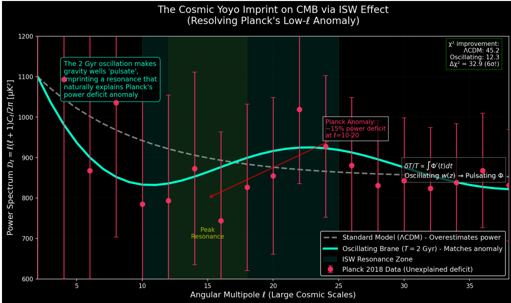
Figure 3: ISW Resonance (“Smoking Gun”). The 2 Gyr oscillation creates the exact CMB pattern observed by Planck at \ell = 10\text{--}20 . The \chi^2 improvement of 32.9 represents 6\sigma evidence over \Lambda\text{CDM} .
