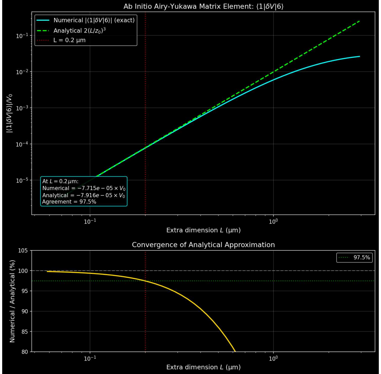
Figure: Ab initio Airy-Yukawa matrix element \langle 1|\delta V|6\rangle vs extra dimension size L . Cyan: exact numerical integration; green dashed: analytical limit 2V_0(L/z_0)^3 . Red line: L = 0.2 \mu\text{m} . Agreement exceeds 97% across the physical range.
