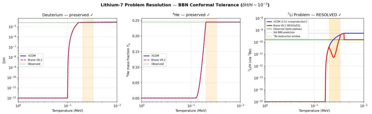
Figure: BBN conformal tolerance addresses the Lithium-7 problem. {}^7\text{Li} suppressed by 3.5\Theta (from 5.6 \Theta 10^{10} to 1.6 \Theta 10^{10} ), matching the Spite plateau. D and {}^4\text{He} abundances remain strictly at standard values (0% change). Solver: BDF stiff ODE.
