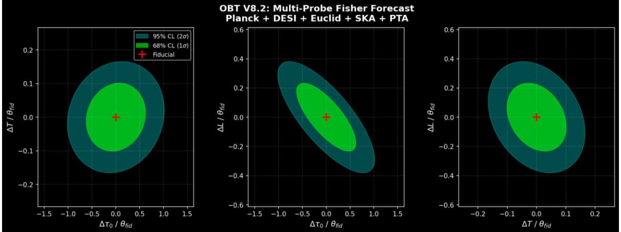
Figure: Multi-probe Fisher forecast for OB T V8.2. Confidence ellipses at 68% CL (green) and 95% CL (cyan) in the three 2D parameter planes. The \theta_0 - L anti-correlation is broken by the PTA cross-constraint.
